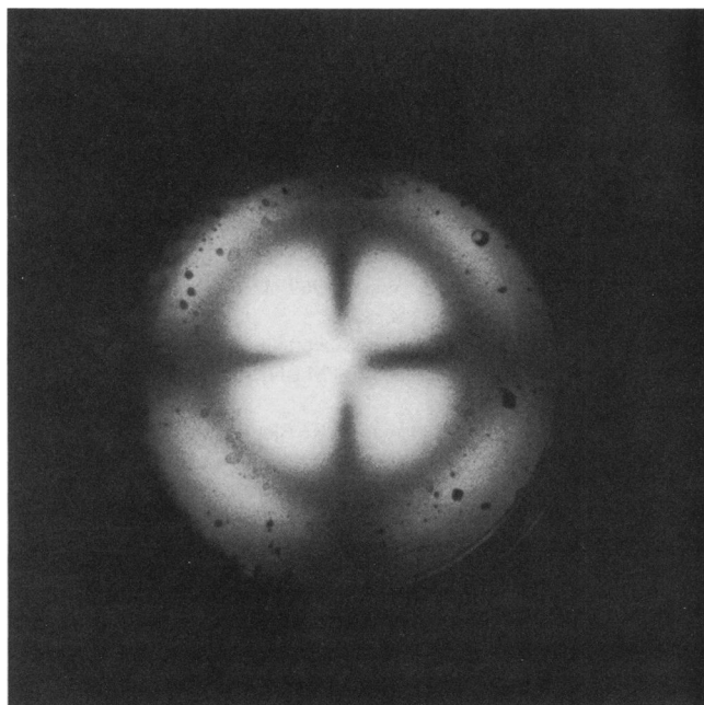
FIGURE 1 Conoscopic interference pattern observed for a 50- \mu\text{m} -thick aligned gramicidin-DLPC sample with a molar ratio of 1:40 and 24% H 2 O by total sample weight. The polarizers were crossed under conoscopic white light illumination. Orientation of the polarizers was the same as the dark cross in the pattern. If it was a color photograph, the rings would be colored with red inside and blue outside. The average index of refraction of the sample was measured (independently) to be 1.443 at \lambda = 632.8 nm. From the radii of the rings, the birefringence \Delta n was calculated to be 0.024 at \lambda = 632.8 nm (20). The center should be dark if the polarizers are perfect. The bubbles (appearing as dark spots) are on the screen and not in the sample.
