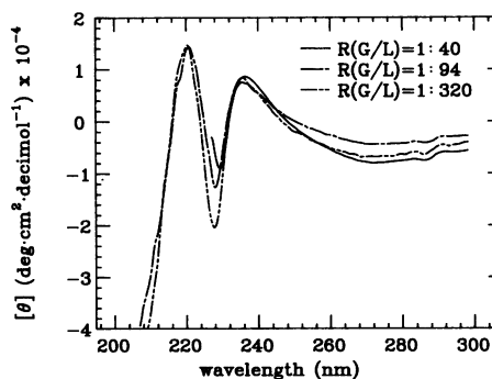
FIGURE 3 CD spectra of gramicidin incorporated in monodomain DLPC multilayers with 20% H 2 O by total sample weight. At R(G/L) \approx 1:40 , strong UV absorption made the spectrum below 225 nm extremely noisy. (This was not a problem for the vesicle suspensions since the UV absorption can be minimized by making the vesicle concentration low.) A mean molecular weight per residue of 124.5 was used to calculate the ellipticities.
